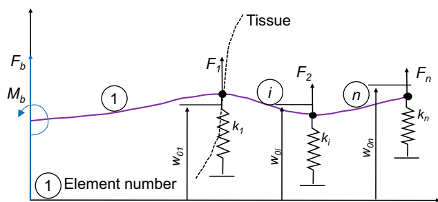
Figure 8 Glozman's beam element and spring model for needle insertion into tissue. Data from DiMaio and Salcudean. 20
