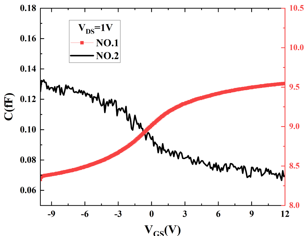
Figure 3 The C-V curve of the present n-type TFTs could be easily changed to that of p-type TFTs.
