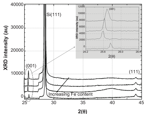
Figure 5 X-ray diffraction patterns for samples with different iron–platinum composition achieved without post-synthesis annealing.
