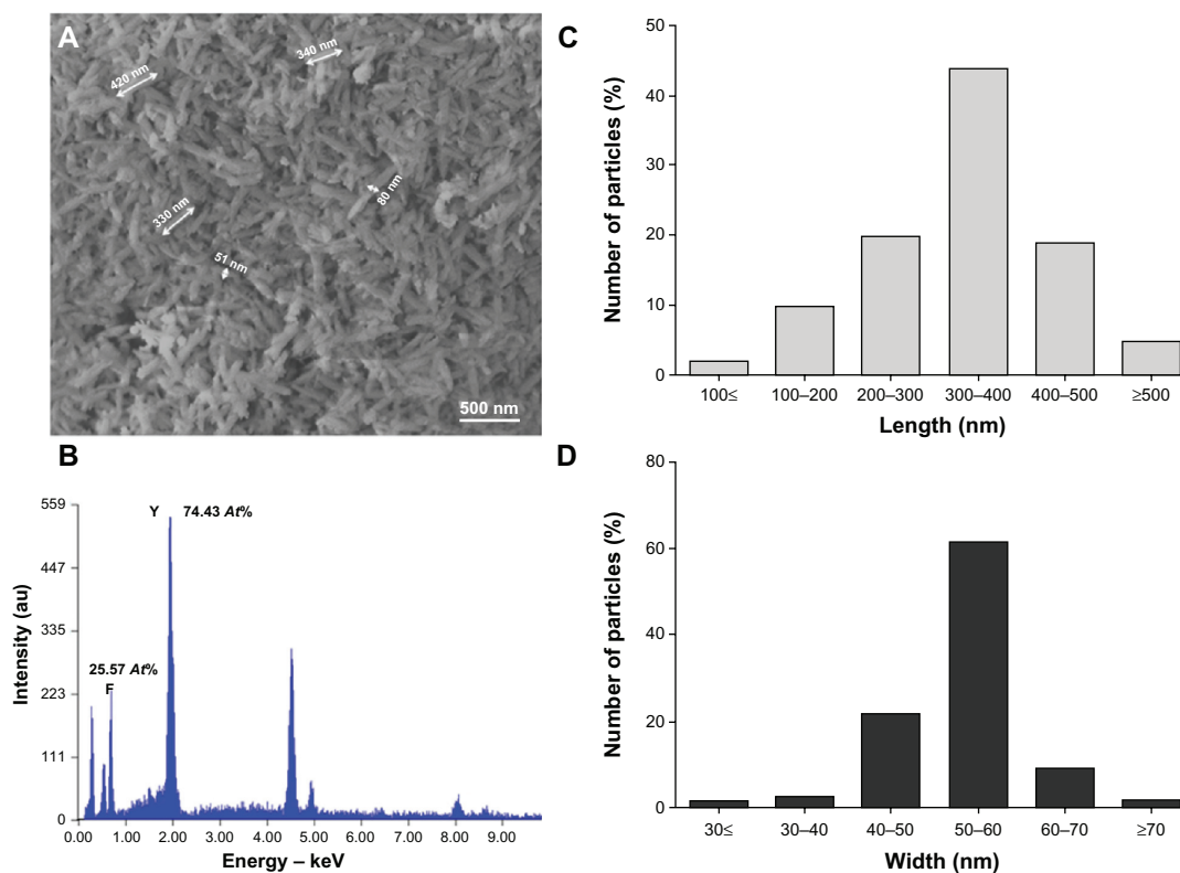
Figure 2 YF_3 NP characterization. (A) SEM micrograph and (B) X-ray elemental spectra of YF_3 NPs. Percentages indicated in (B) refer to the relative atomic ratio between fluorine and yttrium atoms. (C and D) Nanoparticle length and width distributions.
