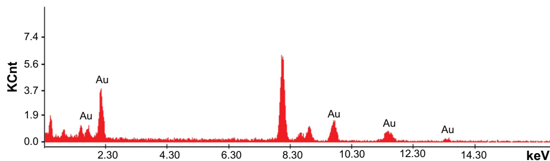
Figure 8 EDAX spectrum of gold nanoparticles. Abbreviation: EDAX, energy dispersive X-ray spectroscopy.
