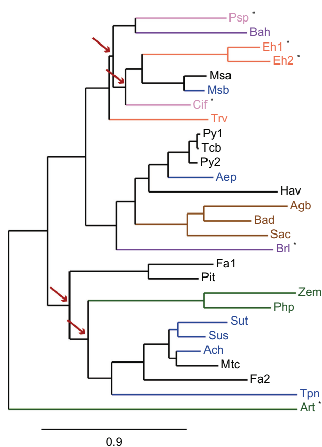
Figure 2 Phylogenetic relationship among methionine-γ-lyases of different species (see Table 1 for strain abbreviations).
