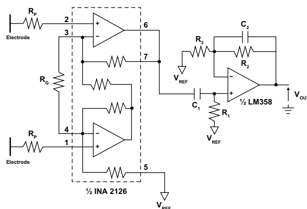
Figure 2 Front end of the electromyograph.
