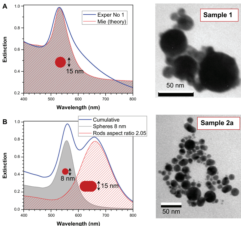
Figure 4 Simulated extinction spectra of less stable solutions No 1 (A) and No 2a (B) with representative transmission electron microscopy images. Assuming 1 cm cuvette length, the concentration of spheres was 9 nM and rods 0.25 nM. The aspect ratio distribution of rods was \sigma = 0.5 . (A) Spectra of sample No 1 (Exper) fitted by: mean radius 15 nm, standard deviation of radius 14 nm, background correction baseline at 0.3 absorbance, total concentration of 530 nM.
