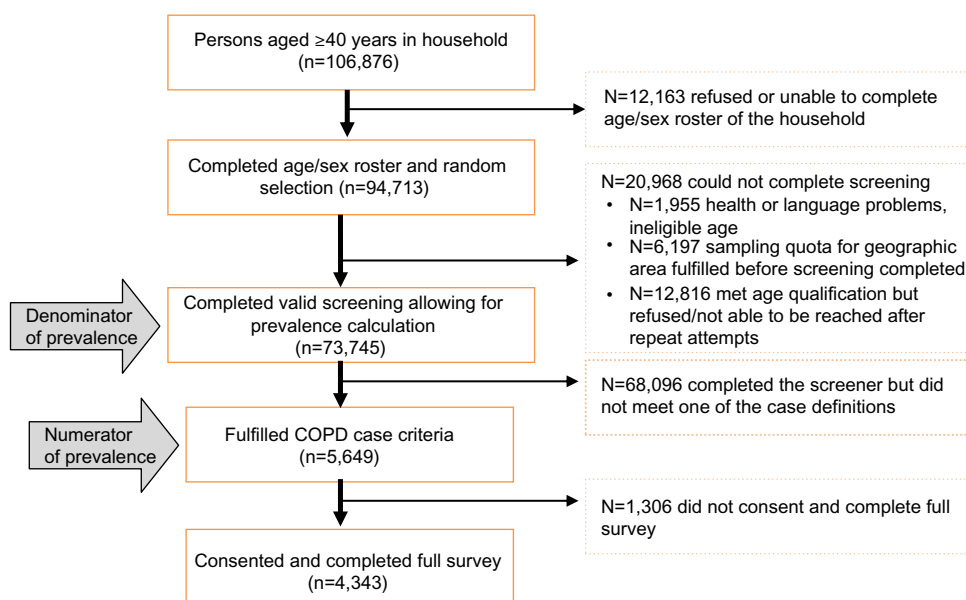
Figure 1 Study-consort diagram.
