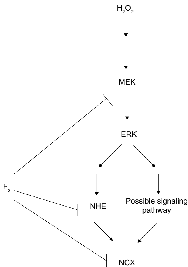
Figure 7 Scheme of possible signaling pathways for NCX activation by \text{H}_2\text{O}_2 and the target of \text{F}_2 action.
