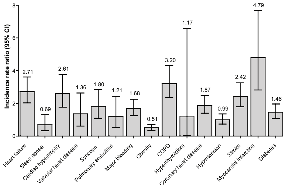
Figure 7 Comparison of incidence rates of all-cause mortality during the postindex period among AF patients with and without baseline comorbidity (MG-EMR data set).
