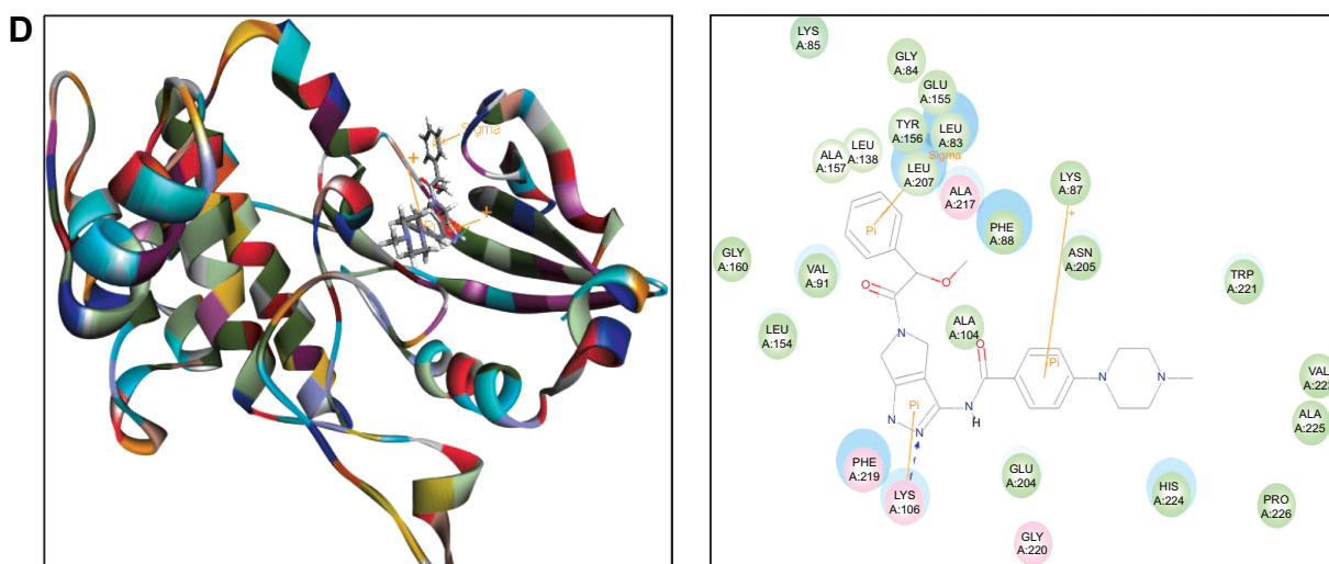
Figure 3 Molecular docking of alisertib, AMG-900, barasertib, CYC116, and danusertib into the active site of human AURKB (PDB ID: 4AF3).
