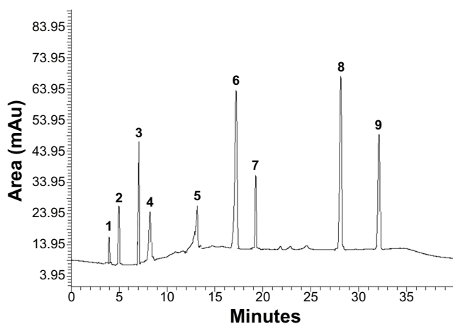
Figure 1 HPLC chromatogram for flavonoids and ascorbic acid standards at 280 nm. Notes: 1) Ascorbic acid; 2) rutin; 3) luteolin; 4) catechin; 5) quercetin; 6) apigenin; 7) naringin; 8) myricetin; and 9) hesperidin. Abbreviation: HPLC, high-performance liquid chromatography.
