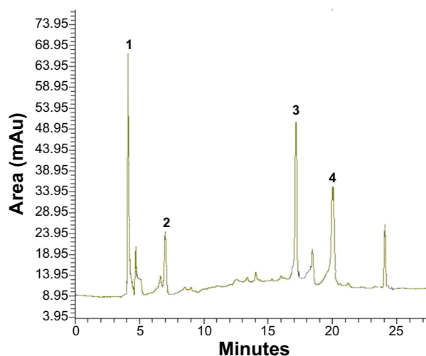
Figure 2 HPLC chromatogram of Basella alba leaves at 280 nm. Notes: 1) Ascorbic acid; 2) luteolin; 3) apigenin; and 4) naringin. Abbreviation: HPLC, high-performance liquid chromatography.
