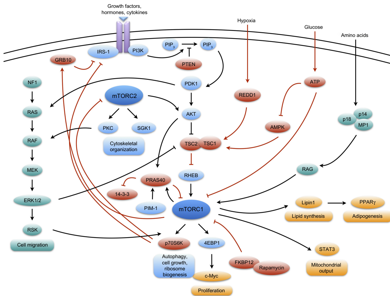
Figure 2 The mTOR signaling pathway.
