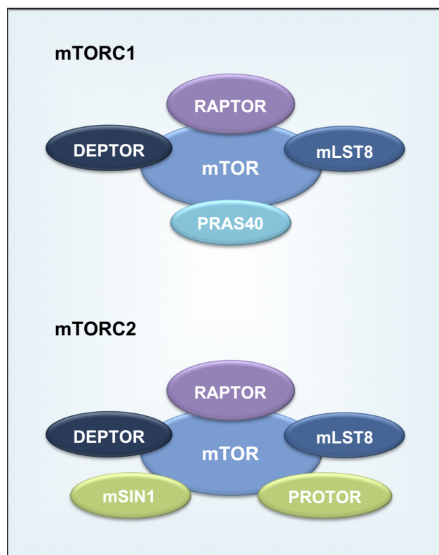
Figure 1 mTORC1 and mTORC2 domains.
