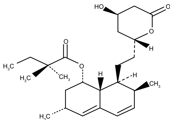
Figure 2 Structural formula for simvastatin.
