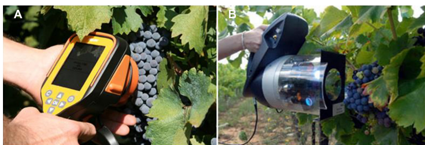
Figure 7 Spectron (A) and Multiplex (B) hand-device sensors for grape quality proximal monitoring, which allows quality maps to be realized.
