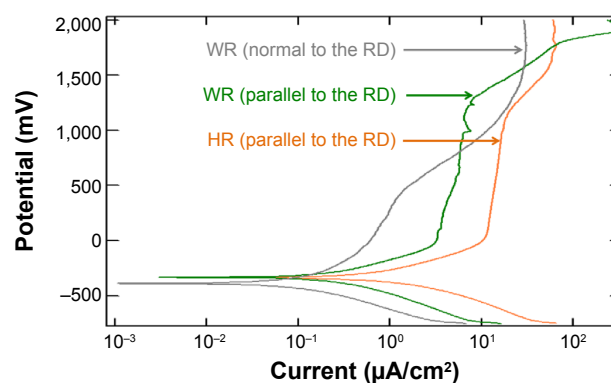
Figure 4 Potentiodynamic curves measured in Hank's solution for the investigated Ti-13Nb-13Zr alloys.
