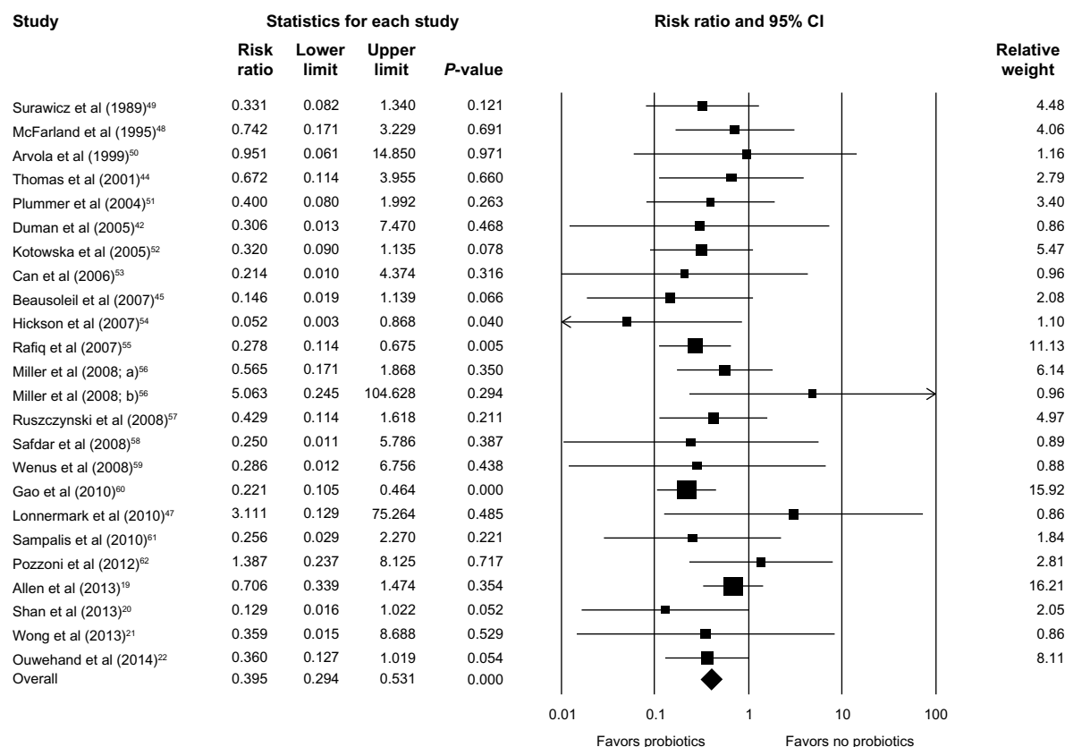
Figure 2 Forest plot evaluating the RR of CDAD associated with probiotic use.
