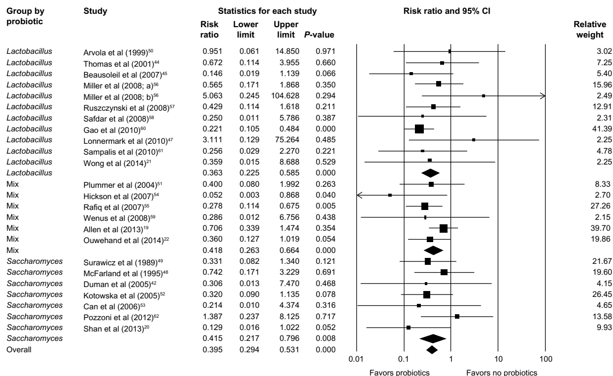
Figure 3 Forest plot evaluating the RR of CDAD associated with various species of probiotic use.
