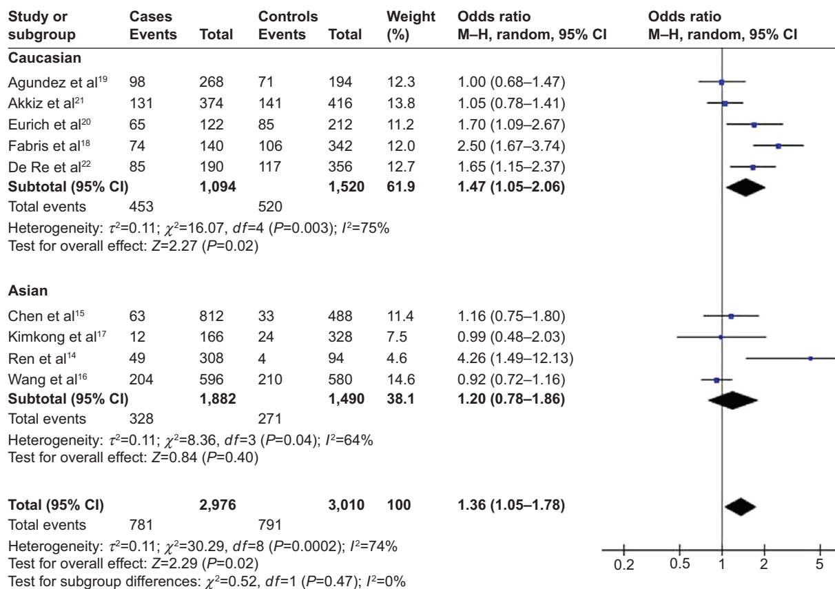
Figure 3 Forest plot describing the association between rs12979860 polymorphism and hepatocellular carcinoma risk (T-allele versus C-allele).
