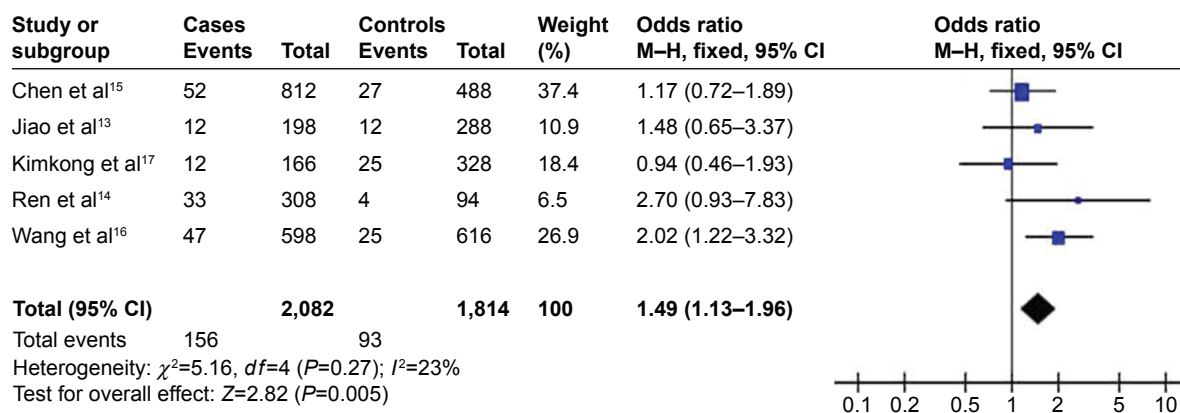
Figure 2 Forest plot describing the association between rs8099917 polymorphism and hepatocellular carcinoma risk (G-allele versus T-allele).
