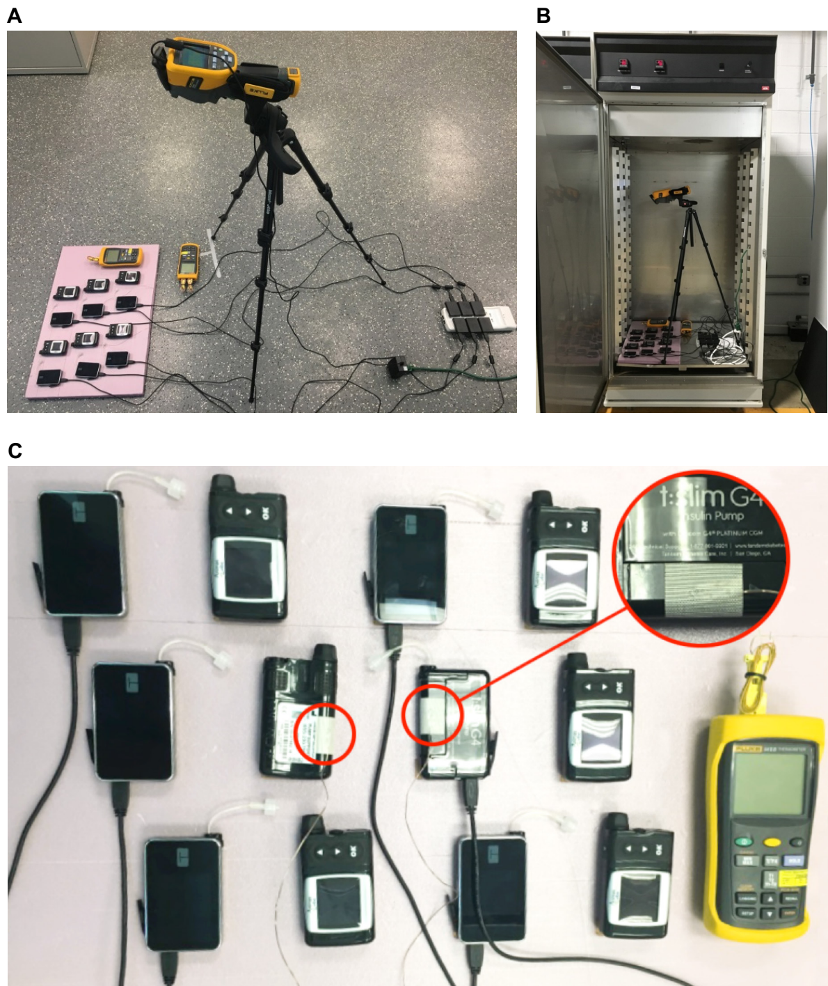
Figure 1 Ambient (A) and environmental-chamber (B) temperature-measurement set up and sensor placement (C).
