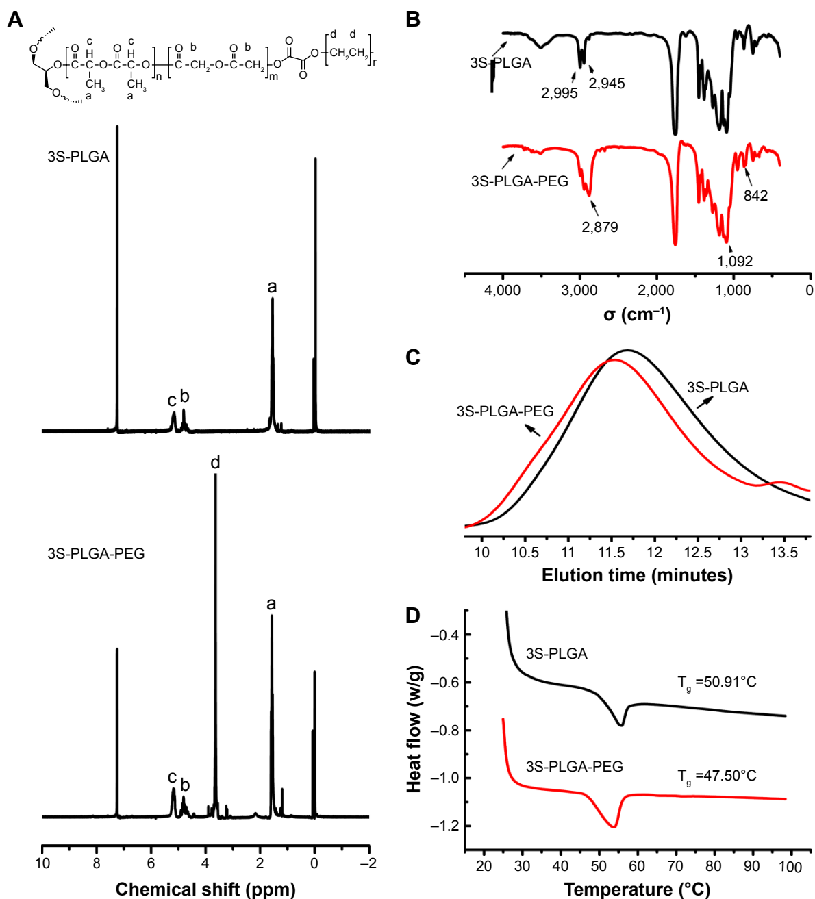
Figure 3 (A) The chemical structure of 3S-PLGA-PEG was investigated by 1 H-NMR spectra. 3S-PLGA was mainly determined by the appearance of the peaks of a ( \delta=1.55 ppm, -CH 3 in PLGA segments), b ( \delta=4.82 ppm, -CH 2 in PLGA segments), and c ( \delta=5.12 ppm, -CH in PLGA segments). Compared with the 3S-PLGA spectrum, the high intensity of peak d ( \delta=3.62 ppm, -CH 2 in PEG segments) in the 3S-PLGA-PEG spectrum indicated the existence of PEG, which proved that 3S-PLGA-PEG was successfully synthesized. (B) FT-IR spectrometry: the characteristic peak of 3S-PLGA at 1,750\text{ cm}^{-1} was attributable to the C=O functional group, while the peaks at 2,995\text{ cm}^{-1} and 2,945\text{ cm}^{-1} were due to the stretching vibration of a saturated -CH bond. In the spectrum of 3S-PLGA-PEG, the emerging peaks of 2,879\text{ cm}^{-1} , 1,092\text{ cm}^{-1} , and 842\text{ cm}^{-1} proved the existence of the PEG chain. (C) Molecular weights and polydispersity were investigated by GPC: the peak of 3S-PLGA-PEG appeared earlier than the peak of 3S-PLGA, which proved that PEG was favorably linked with 3S-PLGA. (D) The glass transition temperature (T g ) of 3S-PLGA was about 50.91^\circ\text{C} , while 3S-PLGA-PEG was 47.5^\circ\text{C} . The existence of PEG affected the crystalline property of PLGA, which reduced the T g of this polymer.
