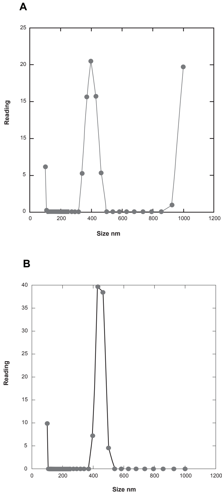
Figure 5 Photonic correlation analysis of superparamagnetic particles used in the present assay. A) Detection angle 60^\circ . B) Detection angle 90^\circ . For experimental details, please see text.
