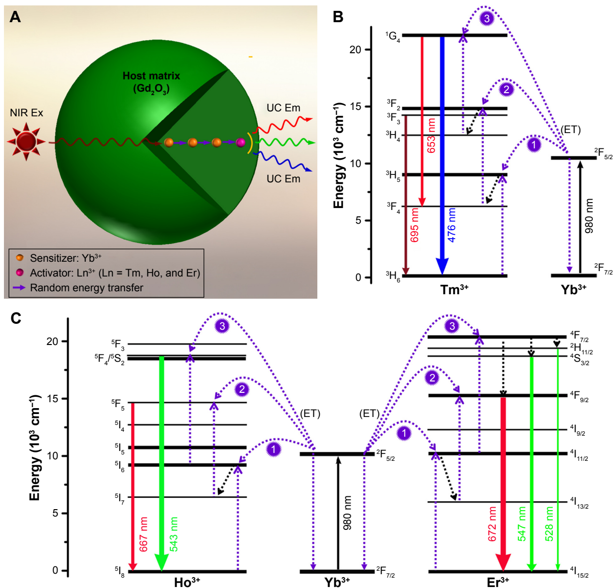
Figure S1 Schematic illustration of the UC emission process ( A ), and the proposed UC mechanism schemes ( B , C ) of the Gd 2 O 3 :Yb 3+ /Ln 3+ (Ln = Tm, Ho, and Er) UCNs. Abbreviations: NIR, near-infrared; UC, upconversion; ET, energy transfer; Ex, excitation; Em, emission.
