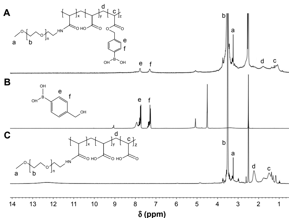
Figure 2 1 H NMR spectra of (A) PPH, (B) HPBA, and (C) PP in DMSO- d 6 .
