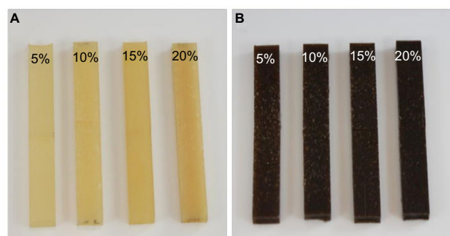
Figure 2 Uncoated and barium-coated HNTs (5%–20%).
