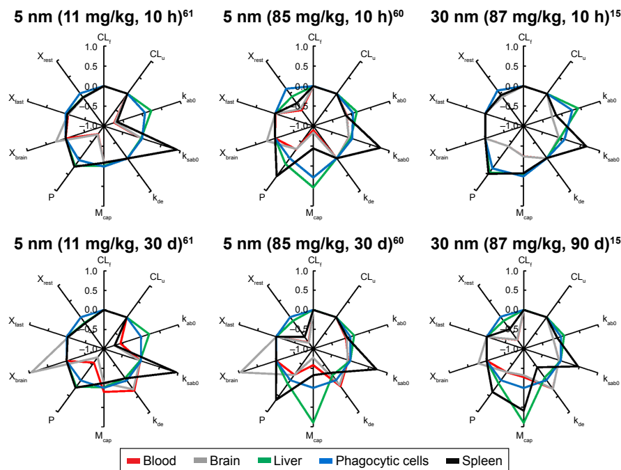
Figure 4 Sensitivity analyses of the physiologically based pharmacokinetic (PBPK) model calibrated with 5 and 30 nm ceria administered intravenously to rats. Notes: Normalized sensitivity coefficients for nanoparticle-specific parameters in blood, liver, spleen, brain, and phagocytic cell compartments are given for 10 h after dosing and at the end of the experiment (30 d for 5 nm and 90 d for 30 nm). Experimental data used for modeling are from Yokel et al. 15,61 Abbreviations: CL_u , clearance rate constant to feces; CL_u , clearance rate constant to urine; k_{abo} , uptake rate constant by phagocytic cells; k_{sabo} , uptake rate constant by phagocytic cells in spleen; k_{de} , exocytosis rate constant from phagocytic cells; M_{cap} , maximum uptake capacity per phagocytic cell; P , partition coefficient between blood and tissue; X_{liver} , coefficient of permeability from blood to liver, spleen, and bone marrow; X_{rest} , coefficient of permeability from blood to lung, kidney, heart, and carcass; X_{brain} , coefficient of permeability from blood to brain.
