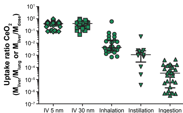
Figure 8 Uptake ratio of nanoceria to liver from different exposure routes. Notes: Translocation of nanoceria from lung and gastrointestinal tract was calculated by dividing the cerium mass in liver with the administered dose, expressed as mass, that is, the uptake ratio. For inhalation, the cerium lung burden was used as the dose. For intravenous (IV) administration, the uptake ratio was calculated as the mass in liver divided by the administered dose. The symbols represent different data sets, and the colors represent different organs.
