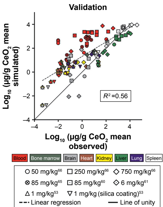
Figure 7 Validation of the physiologically based pharmacokinetic (PBPK) model against independent data sets with 30 nm ceria administered intravenously into rats. Notes: Comparison of logs of simulated and observed mean concentration in different tissues. The line of unity (solid) represents a perfect match, and the regression line (R 2 , dashed) describes the outcome. Different shapes/symbols represent different data sets and colors symbolize organs. Data from Konduru et al, 53 Yokel et al, 60,61,66 and Dan et al. 65
