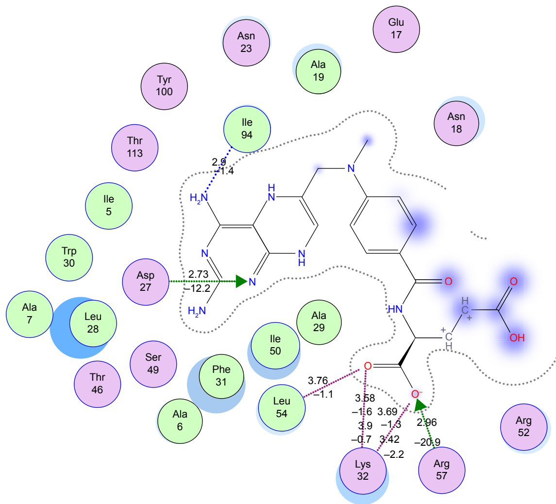
Figure 5 Two-dimensional representation showed interactions of native inhibitor MTX and the DHFR enzyme pocket amino acids. Abbreviations: DHFR, dihydrofolate reductase; MTX, methotrexate.
