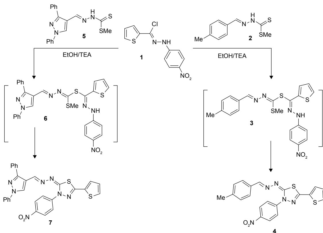
Scheme 1 Synthesis of 1,3,4-thiazazole derivatives 4 and 7.
