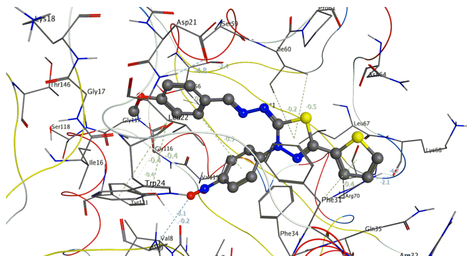
Figure 4 Three-dimensional representation showed interactions of compound 20b and the DHFR enzyme pocket amino acids. Abbreviation: DHFR, dihydrofolate reductase.
