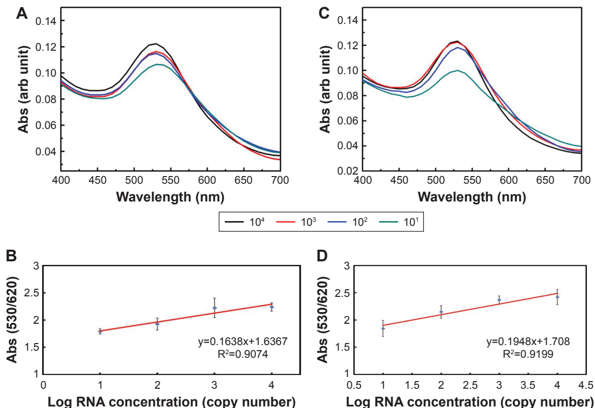
Figure 4 GAG assay spectrum results with TOPI and TDP2 mRNA transcripts. Notes: (A) Different concentrations of TOPI mRNA were detected and quantified by a specific probe using the GAG assay. The mRNA was extracted and then targeted by the conjugated nanoparticles. Different SPRs were obtained according to the TOPI mRNA concentration (copy number). The aggregation behavior was compatible with both SPR and concentration. (B) A standard curve was performed by getting the absorbance ratio ( A_{530}/A_{620} ) against the log of the mRNA concentration. A linear relationship was obtained with R^2=0.9074 . (C) Different concentrations of TDP2 mRNA were targeted by a TDP2-specific probe using the GAG assay according to the TDP2 mRNA concentration (copy number). The aggregation behavior was compatible with both SPR and concentration. (D) A standard curve was performed by plotting the absorbance ratio ( A_{530}/A_{620} ) against the log of the mRNA concentration and a linear relationship was obtained with R^2=0.9199 . Abbreviations: GAG, gold aggregating gold; SPR, surface plasmon resonance; TDP2, tyrosyl DNA phosphodiesterase 2; TOPI, topoisomerase I.
