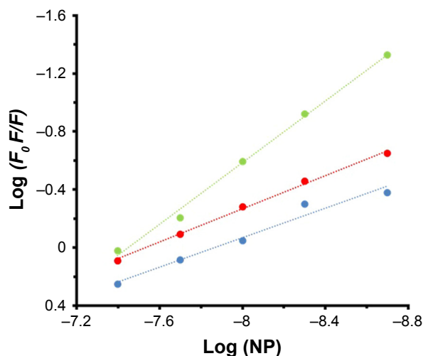
Figure 4 Hill's plot of HSA (2 \mu M) in the presence of varying concentrations of MgO NPs (2, 5, 10, 20, and 40 nM) at three different temperatures of 298K (●), 310K (●), and 315K (●).
