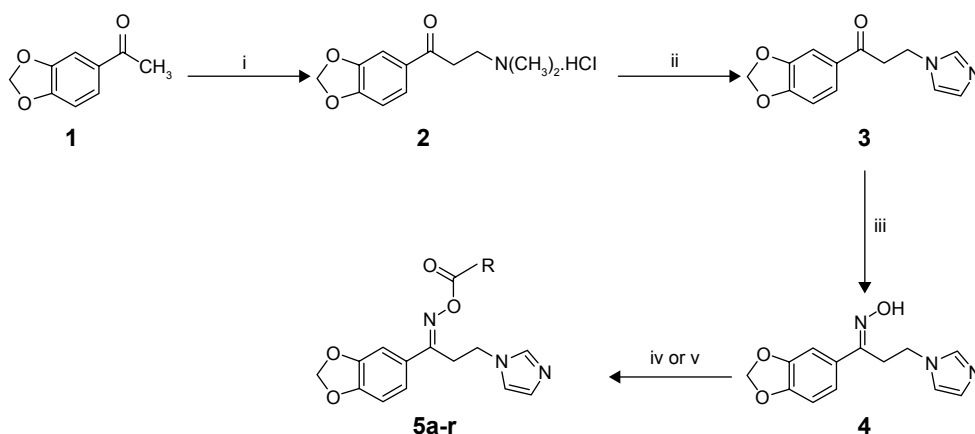
Scheme 1 Synthesis of the target compounds 5a-r . Reagents and conditions: (i) \text{HN}(\text{CH}_3)_2 \cdot \text{HCl} , (\text{CH}_2\text{O})_n , concentrated HCl, ethanol, reflux, 2 hours; (ii) imidazole, water, reflux, 5 hours; (iii) \text{H}_2\text{NOH} \cdot \text{HCl} , KOH, ethanol, reflux, 18 hours; (iv) N,N' -carbonyldiimidazole, ArCOOH, THF, rt, 18 hours, for compounds 5a-d , 5f , 5g , 5i , 5l , 5m , and 5p-r ; and (v) ArCOOH, EDCI.HCl, DMAP, DCM, rt, 18 hours, for compounds 5e , 5h , 5j , 5k , 5n , and 5o .
