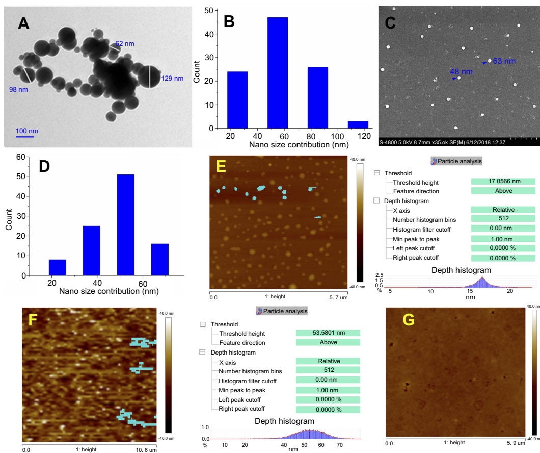
Figure 4 Nano-feature of BCESA in ultrapure water and mouse plasma imaged with TEM, SEM and AFM. (A) Nano-feature of BCESA in ultrapure water (pH 6.8, 0.01 \mu\text{M} ) imaged with TEM; (B) Size distribution of the nano-particles of BCESA in ultrapure water (pH 6.8, 0.01 \mu\text{M} ) imaged with TEM; (C) Nano-feature of the powders lyophilized from a solution of BCESA in ultrapure water (pH 6.8, 0.01 \mu\text{M} ) imaged with SEM; (D) Size distribution of the powders lyophilized from a solution of BCESA in ultrapure water (pH 6.8, 0.01 \mu\text{M} ) imaged with SEM; (E) AFM imaged particles of 17.06 nm in height of BCESA in ultrapure water (pH 6.8, 0.01 \mu\text{M} ); (F) AFM imaged particles of 53.58 nm in height of BCESA in mouse serum (0.01 \mu\text{M} ); (G) AFM image of mouse plasma alone.
