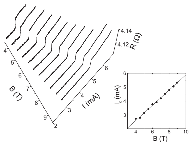
Figure 1 Current-induced excitations at different magnetic fields for a fixed contact size.
