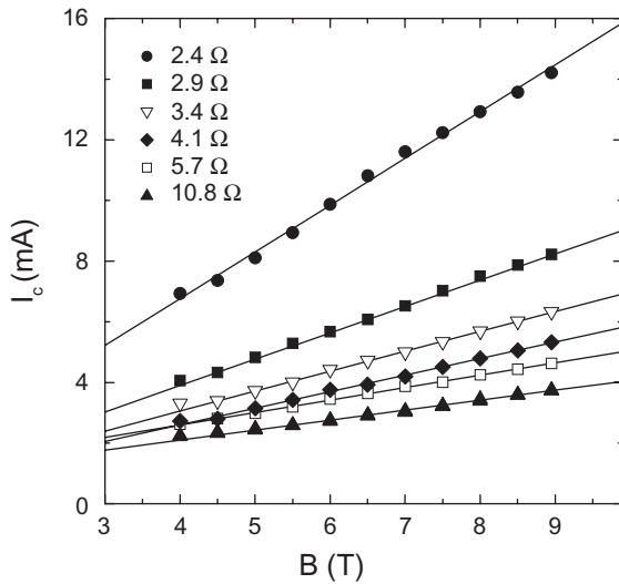
Figure 2 Dependence of critical current I_c(B) for a point-contact of variable size. Notes: Different symbols show the critical current I_c versus applied magnetic field B for a series of point-contact resistances (indicated in the legend). The contact size varies from 8 nm (for R = 10.8 \Omega ) to 24 nm (for R = 2.4 \Omega ). Solid lines are linear fits for I_c(B) s corresponding to different contact resistances.
