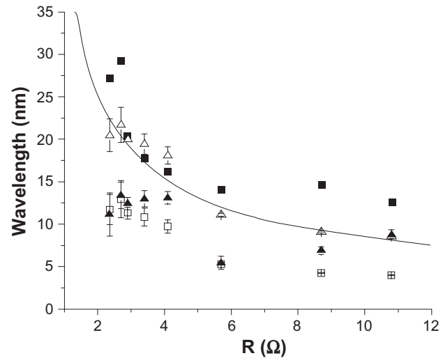
Figure 3 Wavelength \lambda of the current-driven spin waves versus contact (size) resistance R .
