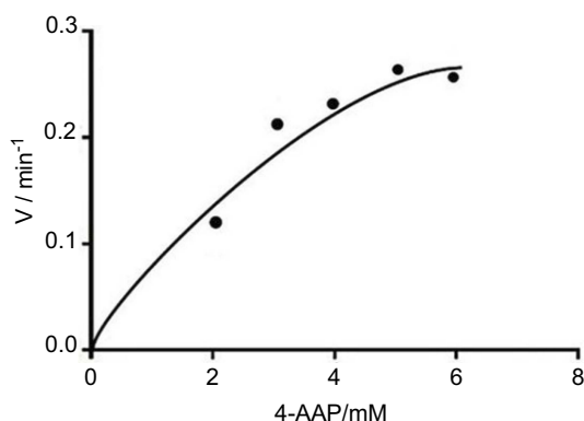
Figure 11 Steady-state kinetic curve based on constant \text{H}_2\text{O}_2 and differed 4-AAP.
