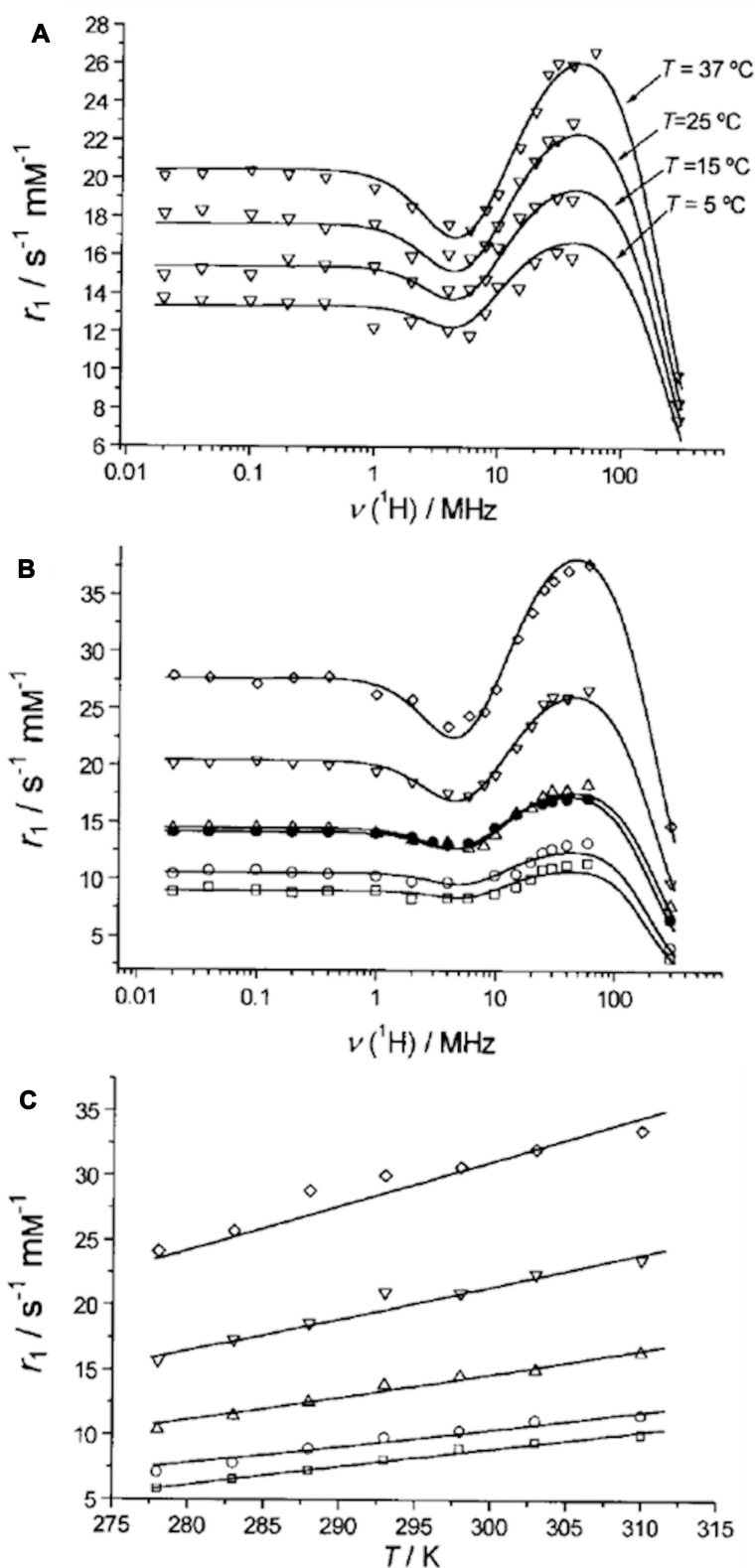
Figure 5 (A) The magnetic field dependence of longitudinal proton relaxation (NMRD profiles) of \text{GdNaY-2.3} recorded at different temperatures. (B) NMRD profiles at different \text{Gd}^{3+} loadings for the \text{GdNaY} samples evaluated at 37^\circ\text{C} . (C) Temperature dependence of the proton relaxivity at 20 \text{ MHz} : \text{GdNaY-1.3} ( \diamond ), \text{GdNaY-2.3} ( \nabla ), \text{GdNaY-3.6} ( \Delta ), \text{GdNaY-5.0} ( \circ ) and \text{GdNaY-5.4} ( \square ) and \text{La-2.8-GdNaY-3.3} ( \bullet ). Reprinted with permission from Platas-Iglesias C, Vander Elst L, Zhou W, et al. Zeolite \text{GdNaY} nanoparticles with very high relaxivity for application as contrast agents in magnetic resonance imaging. Chem Eur J . 2002;8(22):5121–5131. Copyright 2002, John Wiley and Sons. 67
