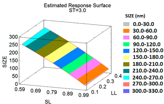
Figure 2 3D response surface plots showing the effects of X1, X2 and X3 on the investigated PSO-NLCs size. Abbreviations: SL, solid lipid; LL, liquid lipid; ST, sonication time.
