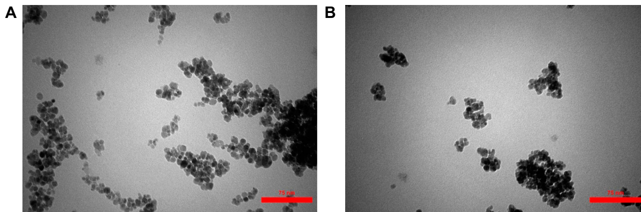
Figure 5 TEM images (a) and (b) of \text{Fe}_3\text{O}_4/\text{SiO}_2/\text{APTS}\text{-Schiff base-Cu(II)} nanoparticles at different magnifications.
