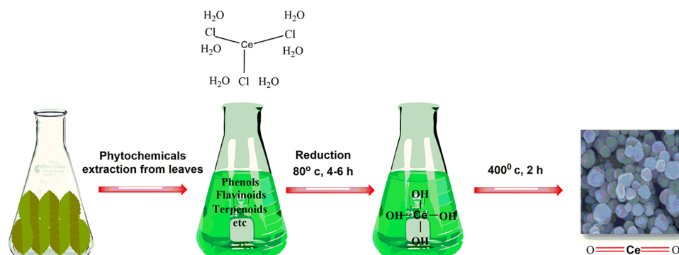
Figure 2 Biosynthesis: Reduction, stabilization and characterization of CeO 2 nanoparticles.
