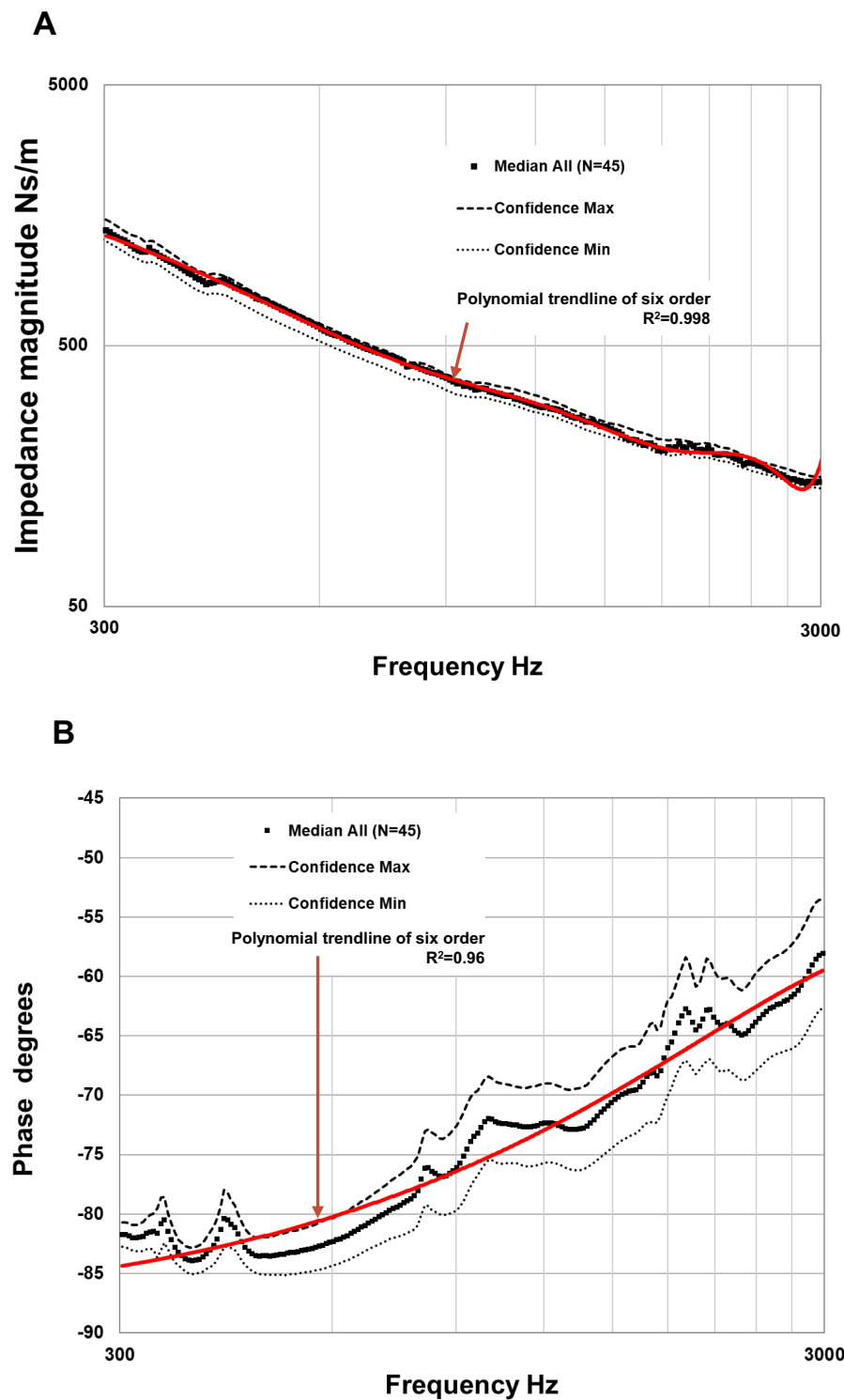
Figure 6 Median magnitude (A) and phase (B) of the skull impedance in the medium frequency region 300–3k Hz of all the 45 subjects tested. The 95% confidence interval is shown as by its max and min values. Trend line of a 6th order polynomials (Excel) was fitted from which parameters were extracted.
