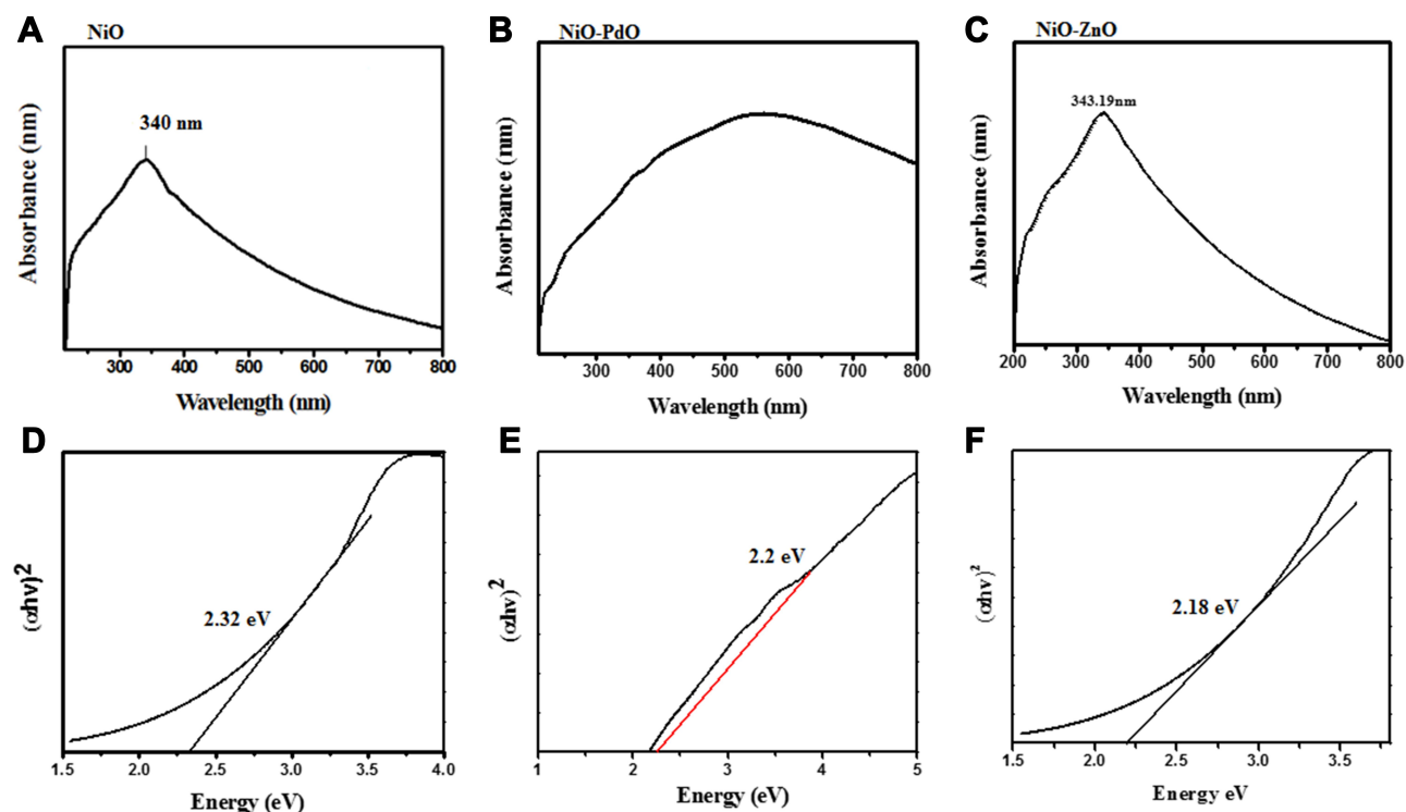
Figure 6 (A–C) Ultraviolet-visible absorption spectra of NiO, NiO–PdO, and NiO–ZnO; (D–F) Tauc plot of energy as ah\nu^2 for NiO, NiO–PdO, and NiO–ZnO.
