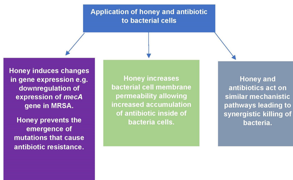
Figure 1 Possible mechanisms by which honey and antibiotics synergistically kill bacterial cells.
