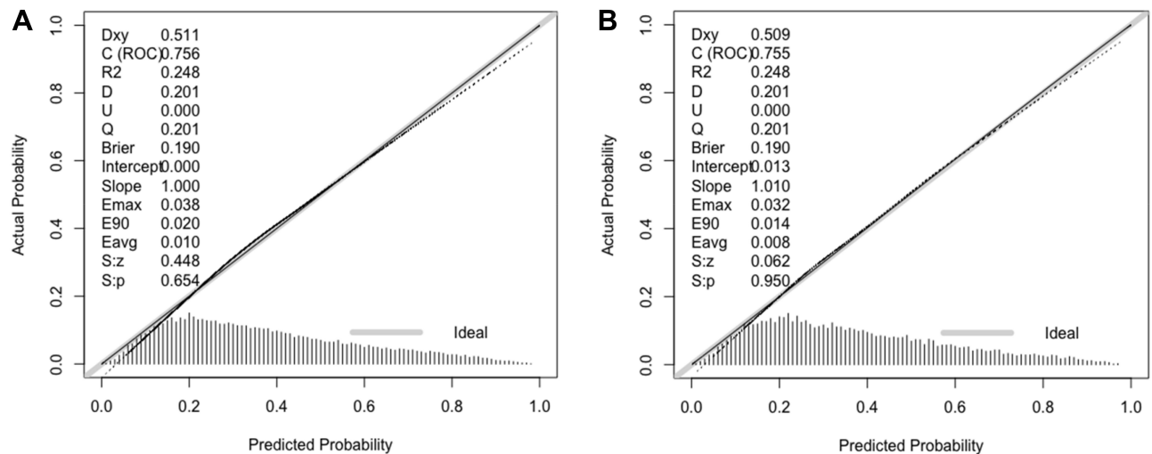
Figure 5 Calibration curves for the prediction and training group models (P = 0.654 vs 0.950).
