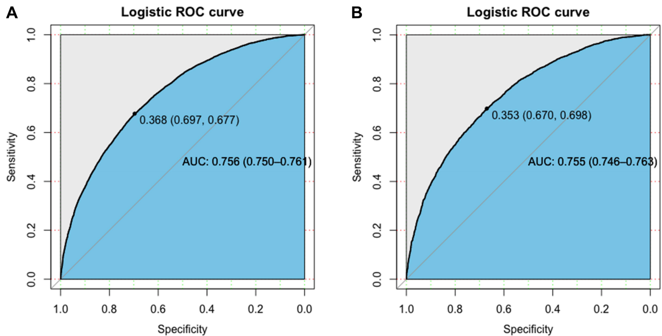
Figure 4 ROCs for validating the discrimination power of the nomogram. (A) Development group. (B) Validation group (AUC = 0.756 vs 0.755).
