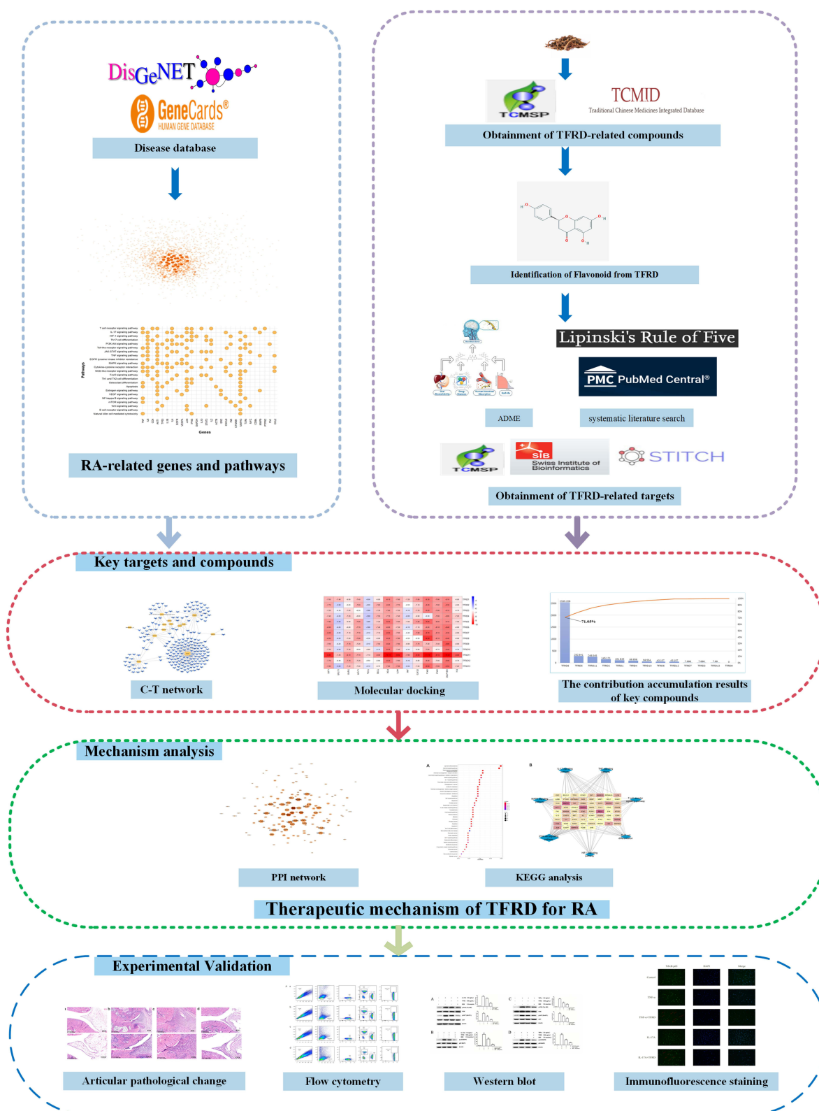
Figure I The flowchart of this study. Network pharmacology approach includes the acquirement of RA-related genes and TFRD-related compounds and targets, construction of C-T network, accumulation of key compounds, PPI network construction, KEGG enrichment analysis, molecular docking. Experimental validation involves pathological images, flow cytometry, Western blotting, immunofluorescence.
