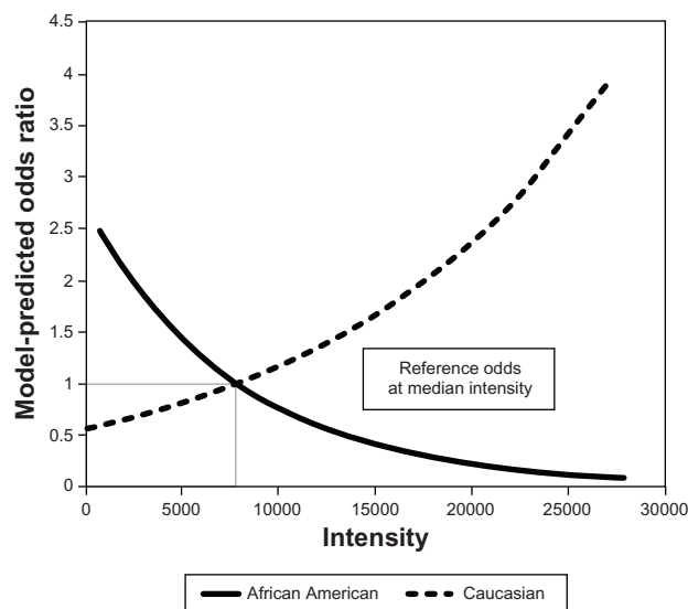
Figure 2 Association between the intensity of peak m/z = 4154 and odds ratio for CIN 2+ for Caucasian Americans a and African Americans. b
