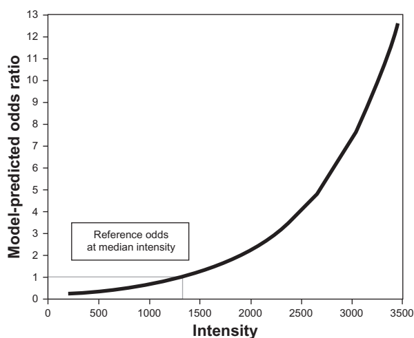
Figure 1 Association between the intensity of peak m/z = 4459 and odds ratio for CIN 2+.
