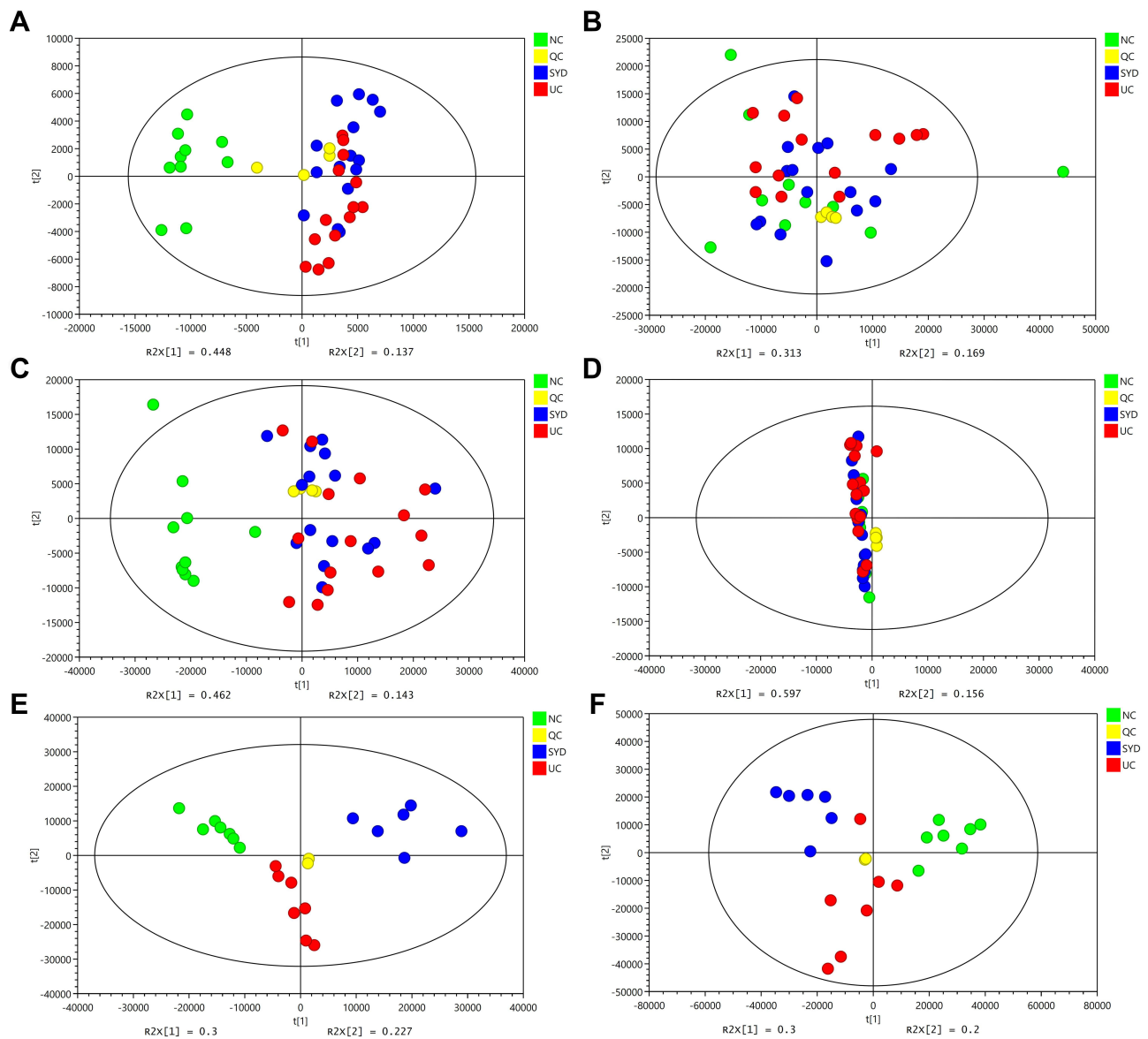
Figure 7 PCA score plots of livers, serum and urine metabolic profiling between normal, model and SYD group. (A) Liver samples detected in positive mode. (B) Liver samples detected in negative mode. (C) Serum samples detected in positive mode. (D) Serum samples in negative mode. (E) Urine samples detected in positive mode. (F) Urine samples detected in negative mode.
