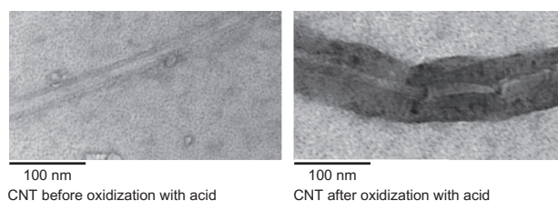
Figure 2 Carbon nanotubes (CNT) before and after oxidization using a combination of nitric and sulfuric acid. This method resulted in chemical modifications of carbon nanotubes and formation of carboxylate groups on the surface.
