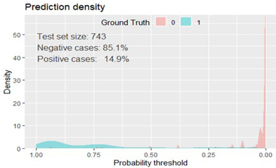
Figure 7 Prediction density plot for developed model using original beta coefficients at UoGCSH, 2012–2022. Abbreviation: UOGCSH, University of Gondar Comprehensive Specialized Hospital.
