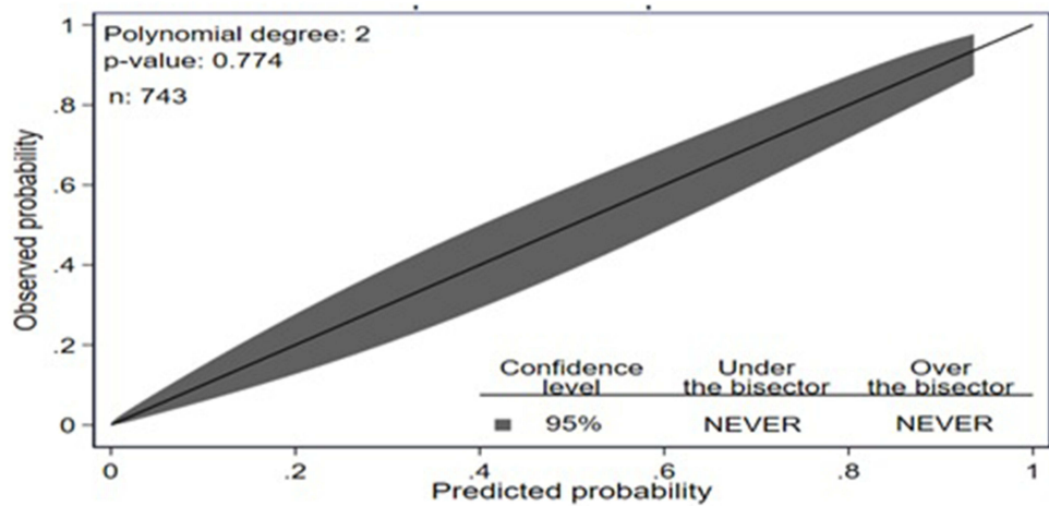
Figure 4 Calibration plot for developed model based on original beta coefficient for stroke prediction model among hypertensive patients at UoGCSH, 2012–2022. Notes: 95% CI calibration belts are plotted in dark gray. The black diagonal line is the reference line indicating perfect calibration. Abbreviation: UOGCSH, University of Gondar Comprehensive Specialized Hospital.
