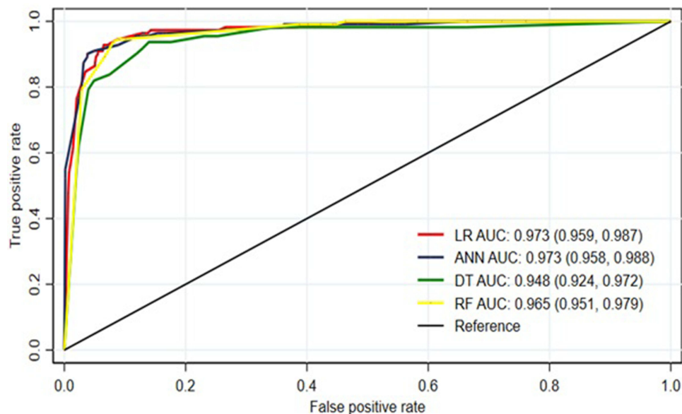
Figure 12 AUROC curves of the machine learning algorithm and multivariable logistic regression at UoGCSH, 2012–2022.
