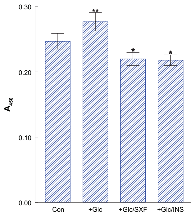
Figure 3 Effects of SXF or INS on IRS-1(s) phosphorylation under high Glc. Notes: Following 24-hour high Glc treatment, cells were exposed to SXF (300 µg/mL) or INS (100 nM) for 15 minutes and IRS-1(s) was analyzed using ELISA. All data are mean ± SD from three separate experiments (* P < 0.05 versus Glc-treated or ** P < 0.05 versus control).
