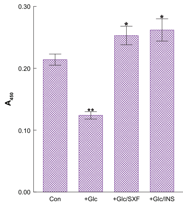
Figure 4 Effects of SXF or INS on Akt(s) phosphorylation under high Glc. Notes: Following 24-hour high Glc treatment, cells were exposed to SXF (300 µg/mL) or INS (100 nM) for 15 minutes and Akt(s) was analyzed using ELISA. All data are mean ± SD from three separate experiments (* P < 0.01 versus Glc-treated or ** P < 0.03 versus control).
