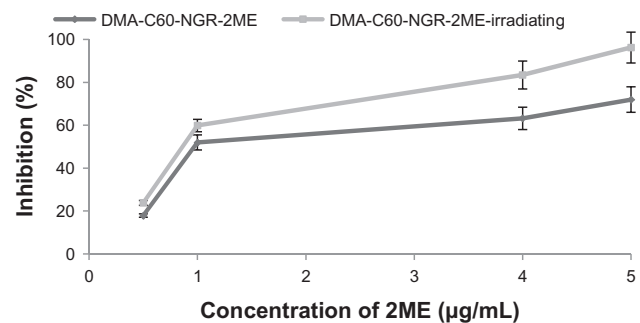
Figure 14 Inhibition efficacy of DMA-C60-2ME-NGR and DMA-C60-2ME-NGR-irradiating group on MCF-7 cells for 24 hours. Note: Data are presented as mean ± standard deviation (n = 3). Abbreviations: DMA-C60, diadduct malonate derivative of C60; NGR, Asn-Gly-Arg peptide; 2ME: 2-methoxyestradiol.
