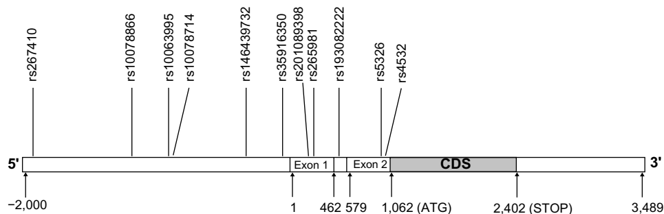
Figure 1 Schematic diagram of the distribution of eleven SNP loci in the DRD1 gene. Abbreviations: CDS, coding sequence; SNP, single nucleotide polymorphism; ATG, transcription start site; STOP, stop codon.
