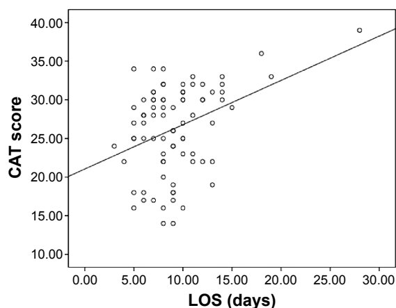
Figure 5 Pearson's correlations between CAT and LOS.
